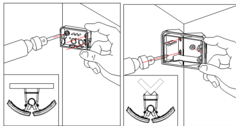
Wandmontage
